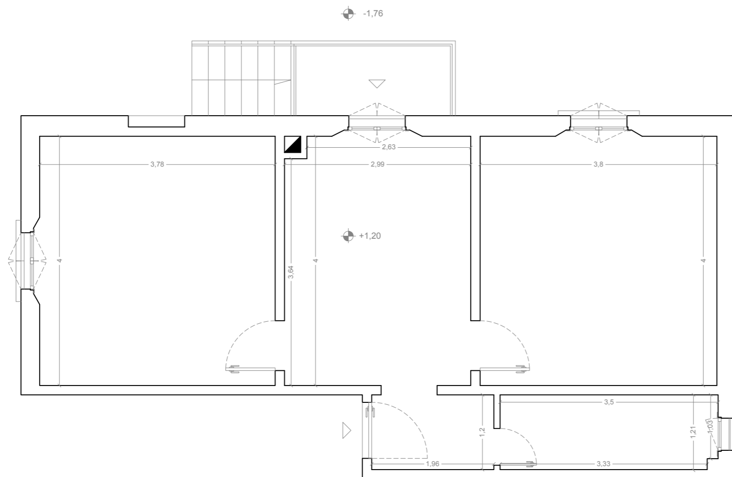
piano terra
